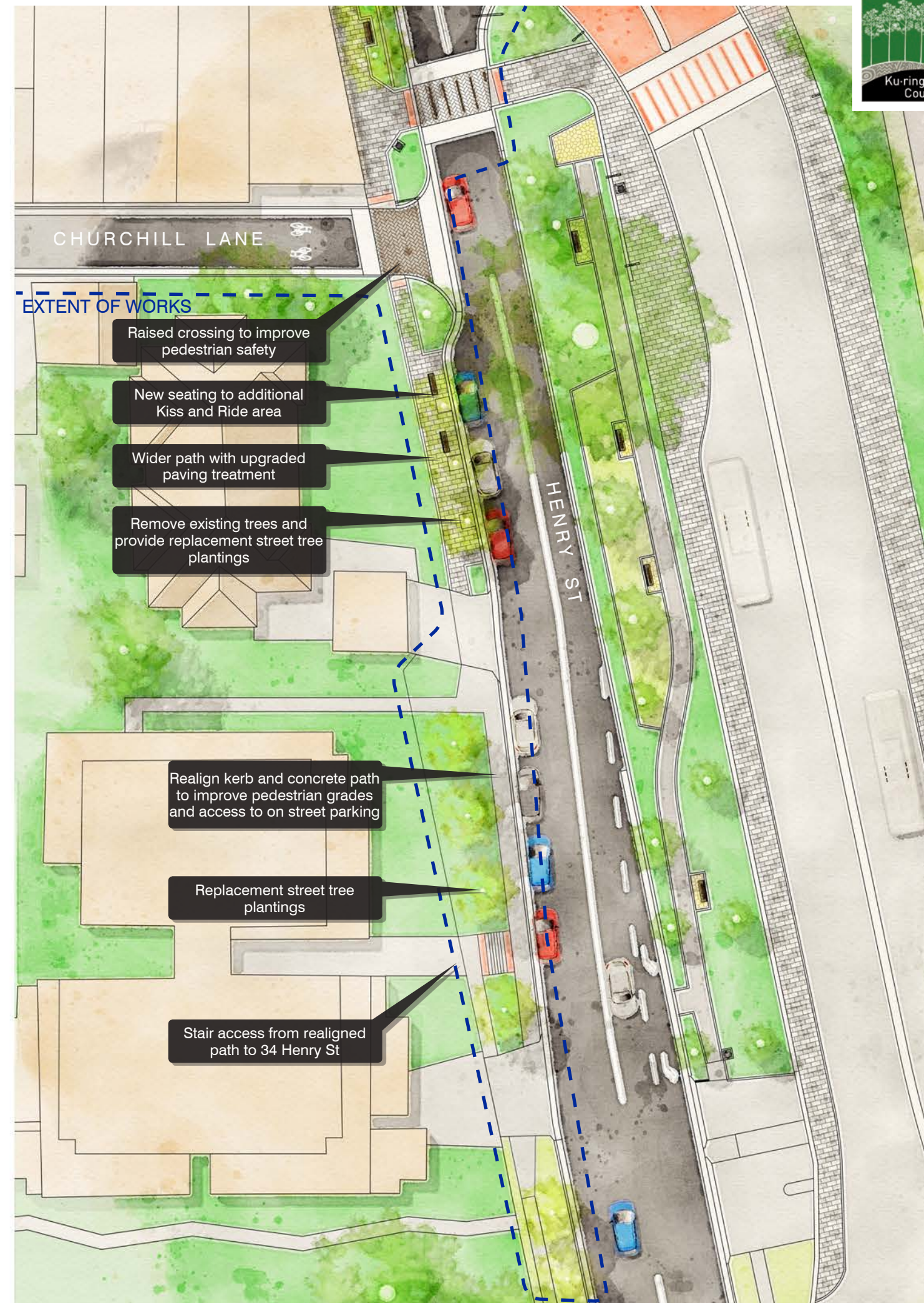
HENRY STREET, GORDON - PROPOSED CONCEPT PLAN
