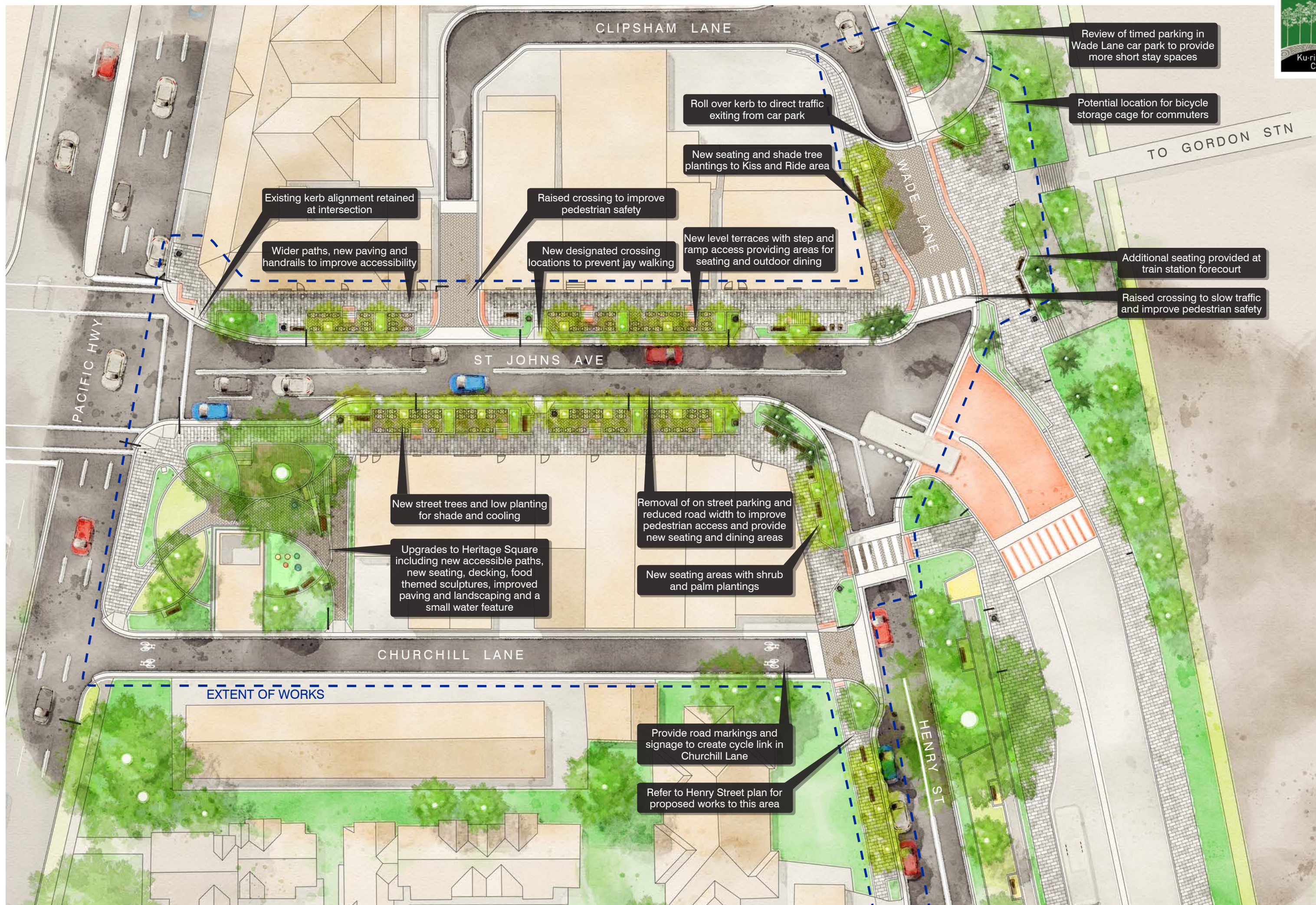
ST JOHNS AVENUE, GORDON - PROPOSED CONCEPT PLAN
