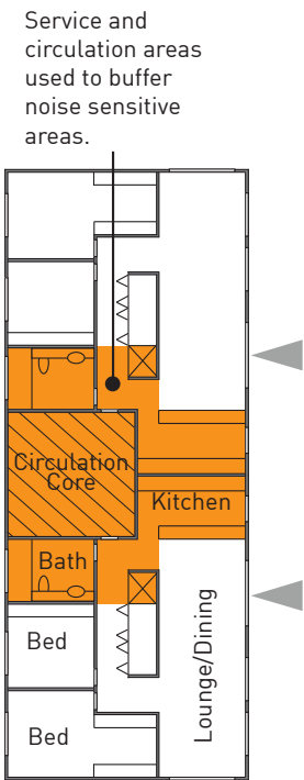
Figure 23.8-1: Buffer zone to minimise noise pollution.
