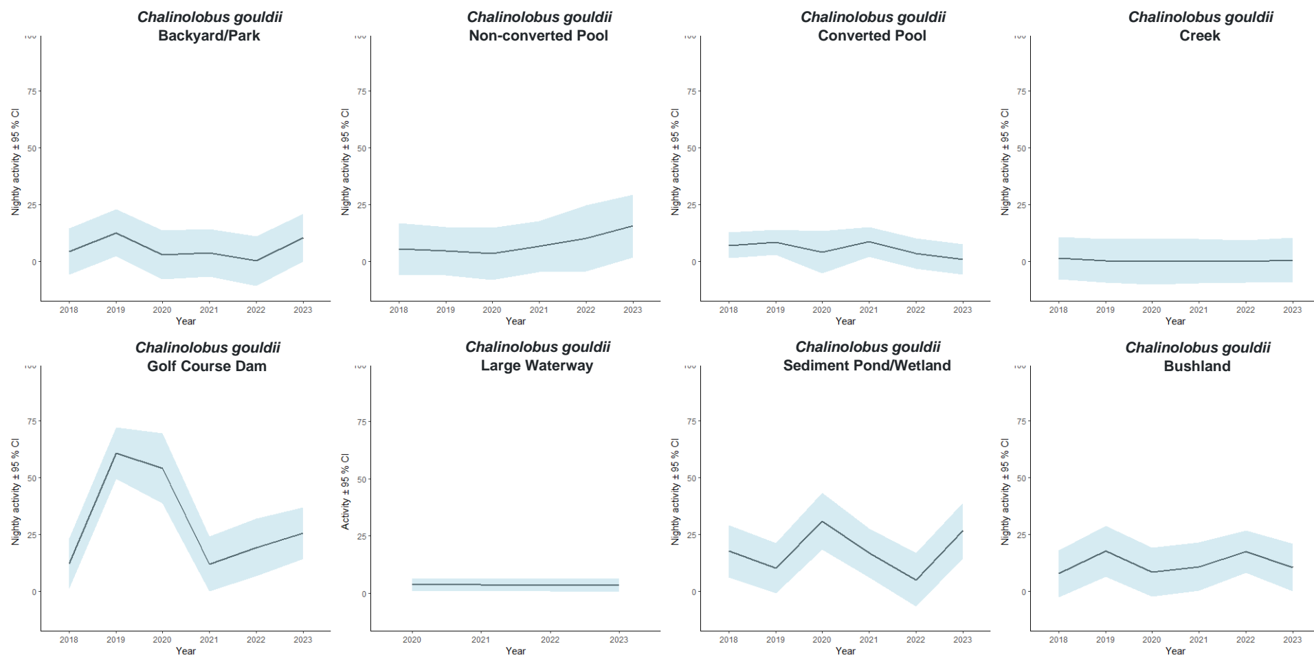
Fig. 7. Nightly Chalinolobus gouldii activity recorded among habitat types in the Ku-ring-gai LGA between 2018 and 2023. Back-transformed estimated means are displayed \pm 95 % confidence intervals.
