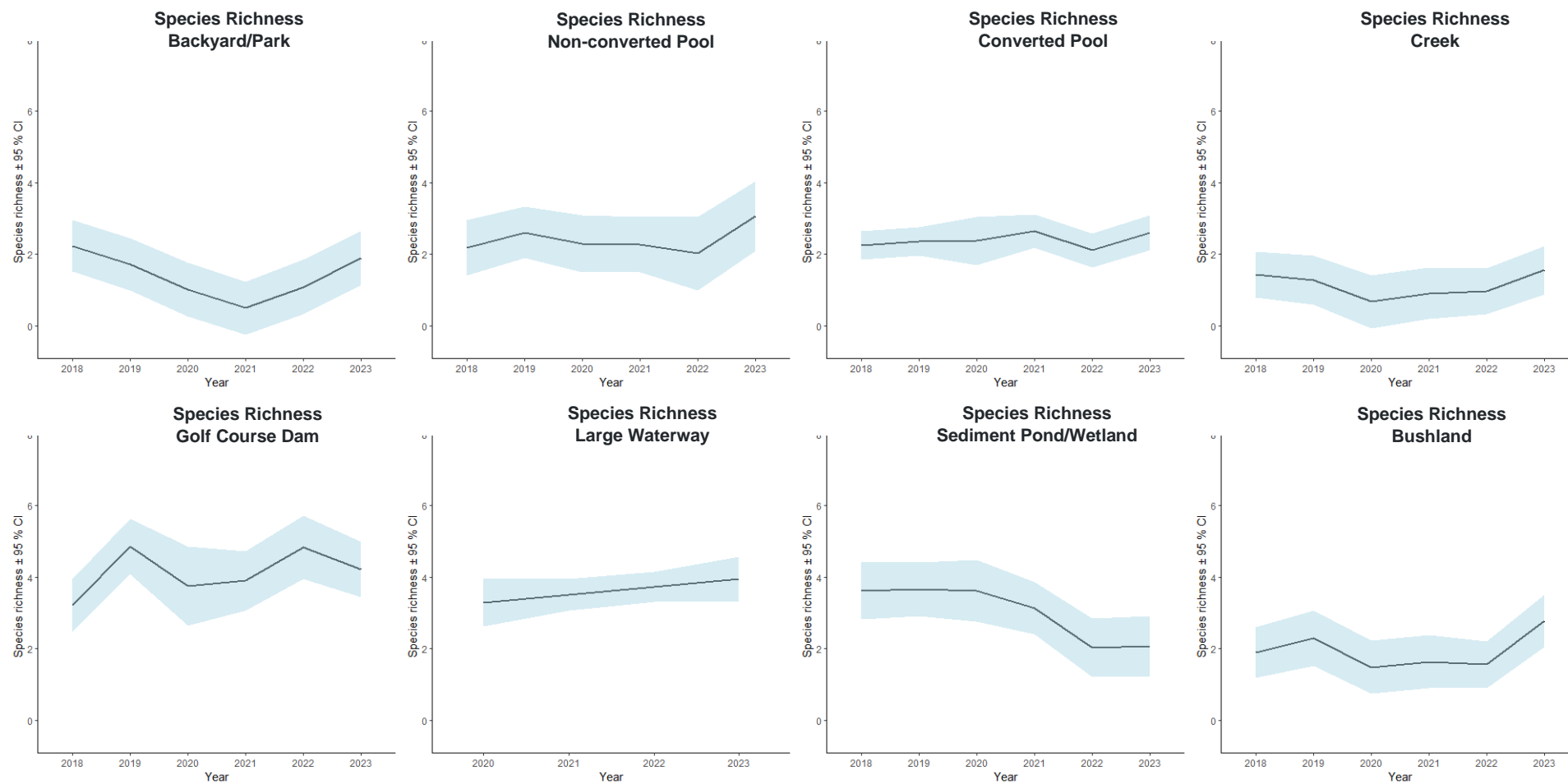
Fig. 4. Nightly bat species richness recorded among habitat types in the Ku-ring-gai LGA between 2018 and 2023. Back-transformed estimated means are displayed \pm 95\% confidence intervals.
