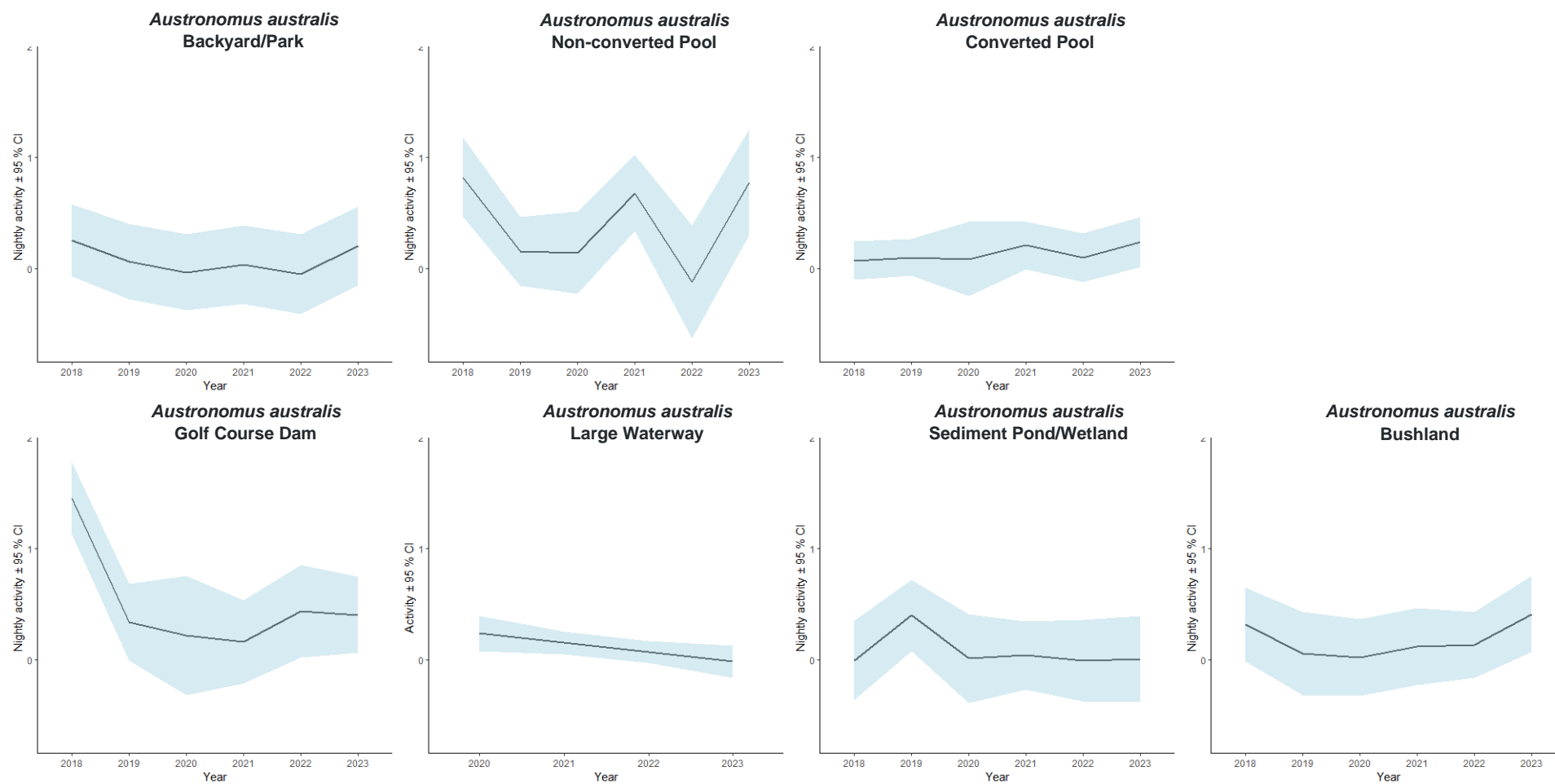
Fig. 6. Nightly Austronomus australis activity recorded among habitat types in the Ku-ring-gai LGA between 2018 and 2023. Back-transformed estimated means are displayed \pm 95 % confidence intervals.
