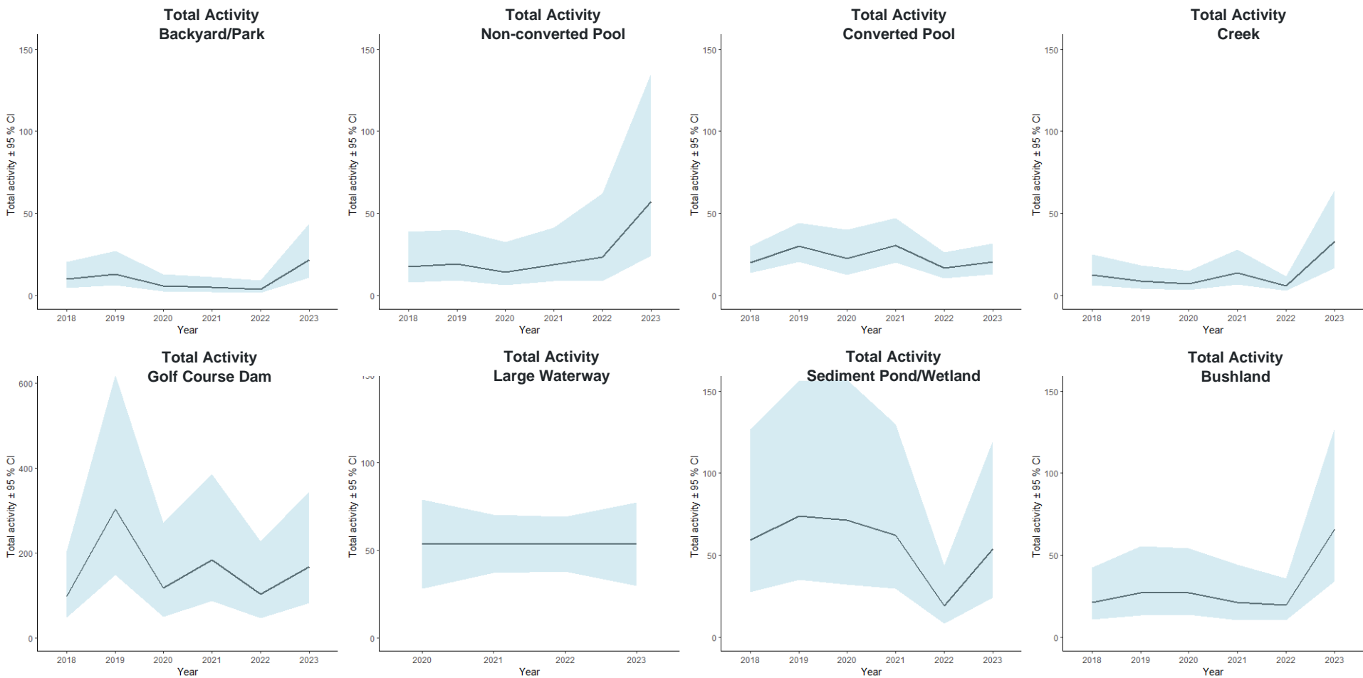
Fig. 5. Nightly bat activity recorded among habitat types in the Ku-ring-gai LGA between 2018 and 2023. Back-transformed estimated means are displayed ± 95 % confidence intervals.
