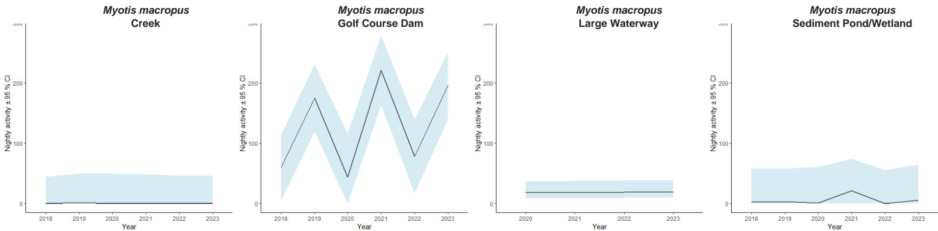
Fig. 9. Nightly Myotis macropus activity recorded among habitat types in the Ku-ring-gai LGA between 2018 and 2023. Back-transformed estimated means are displayed ± 95 % confidence intervals.
