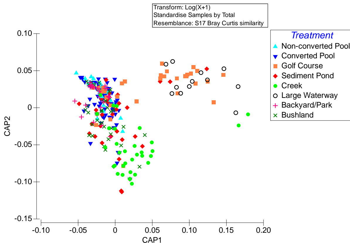
Fig. 11. Canonical analysis of principal coordinates (CAP) plot illustrating differences between habitat types on the basis of bat species assemblages.
