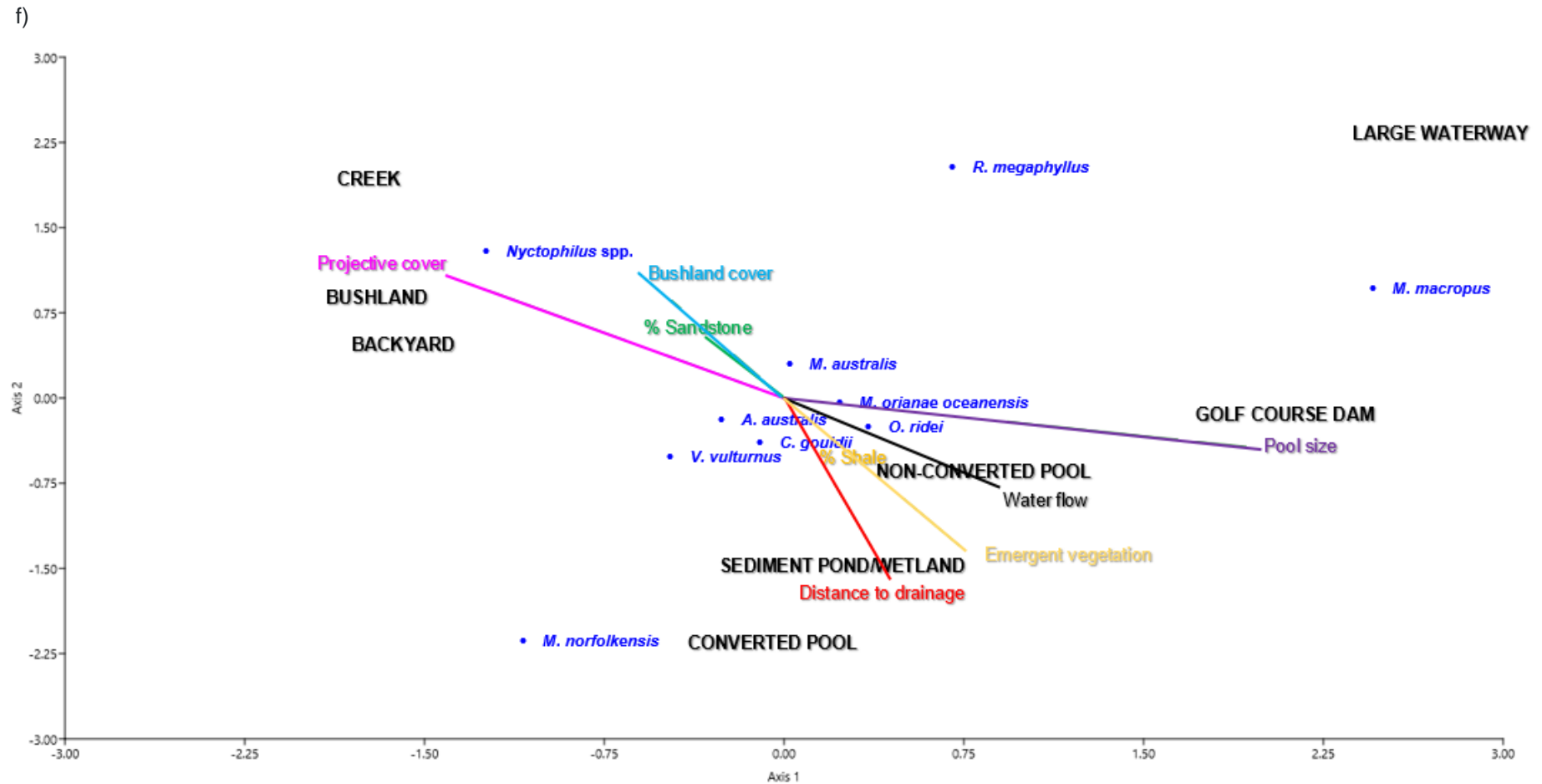
Fig. 12. Canonical correspondence analysis bi-plot illustrating associations between activity of bat taxa and environmental variables in a) 2018, b) 2019, c) 2020, d) 2021, e) 2022 and f) 2023. Centroids for the different habitat types are also plotted.
