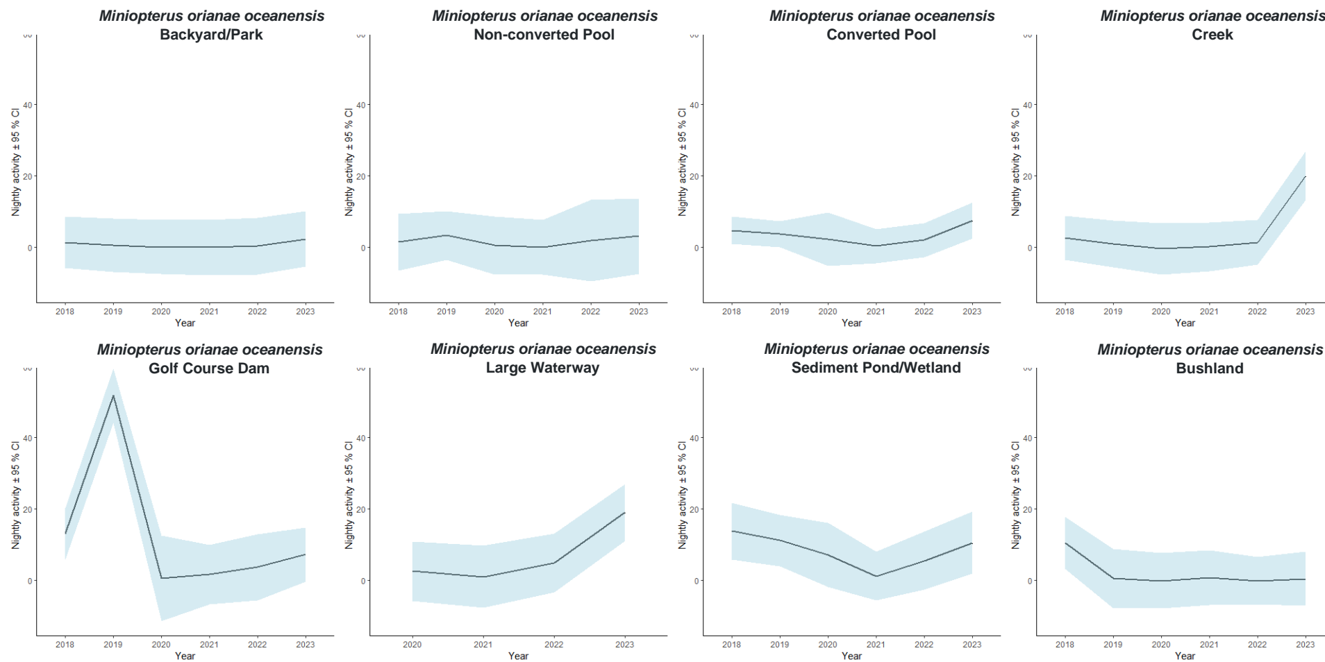
Fig. 8. Nightly Miniopterus orianae oceanensis activity recorded among habitat types in the Ku-ring-gai LGA between 2018 and 2023. Back-transformed estimated means are displayed ± 95 % confidence intervals.
