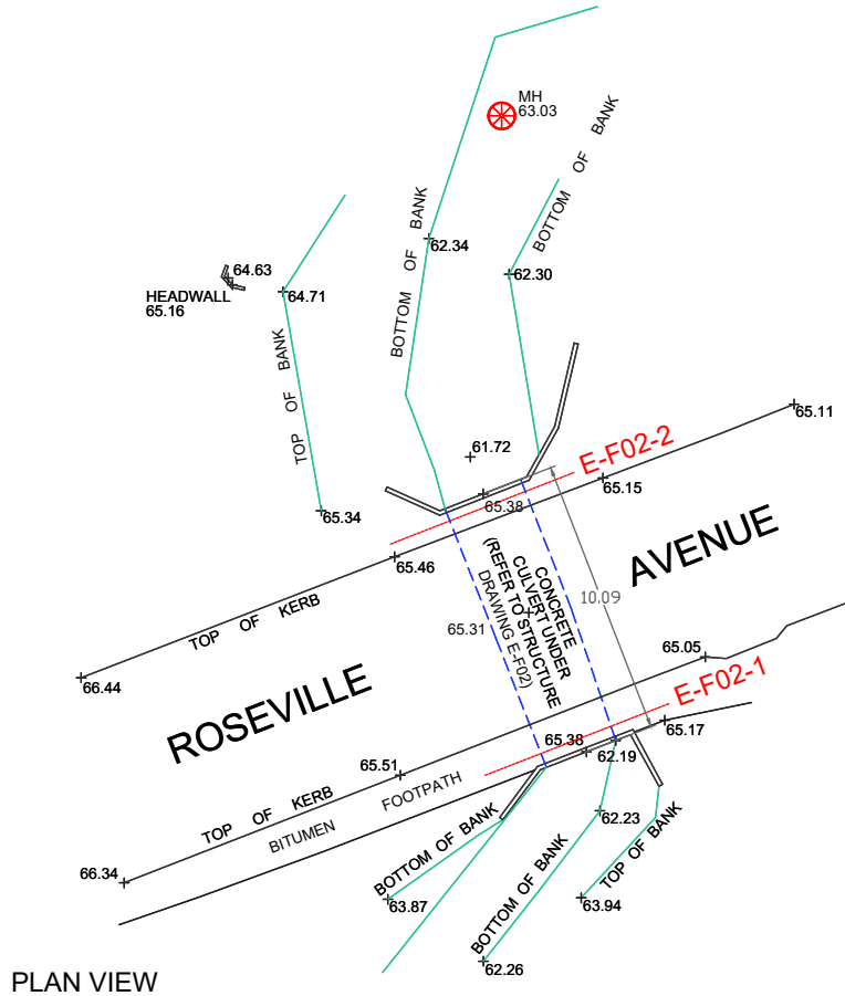
PLAN VIEW
