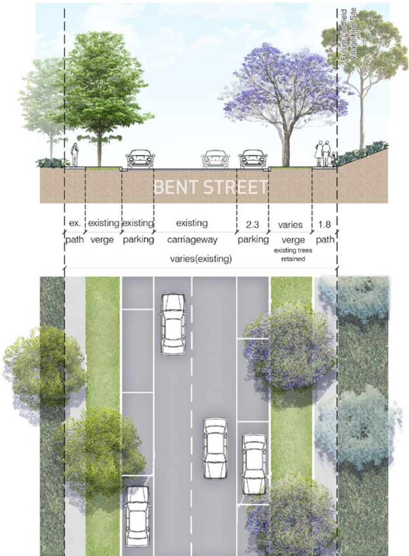
Figure 65: Bent Street Site Section
