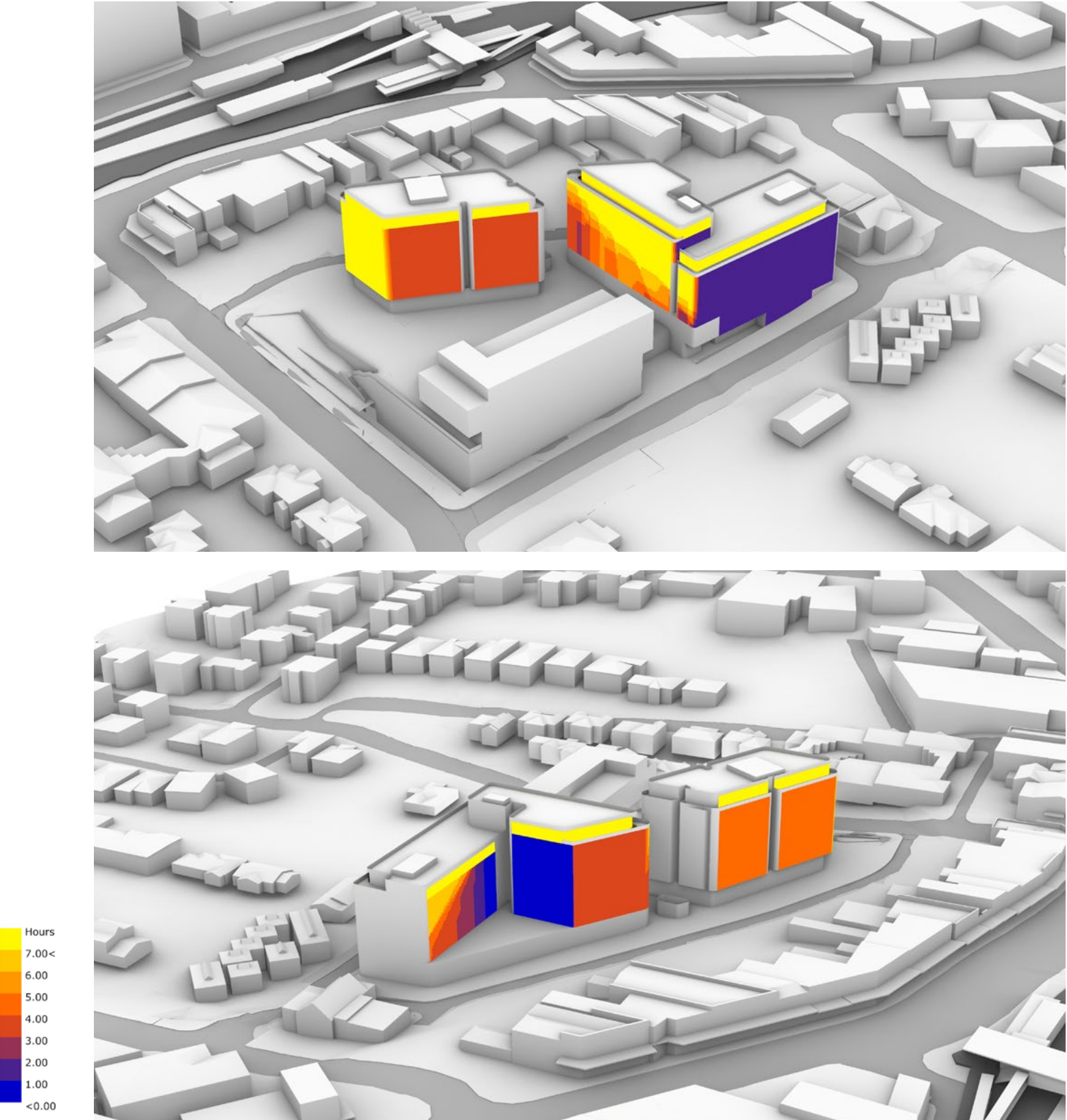
Figure 73: Facade Solar Access Model
