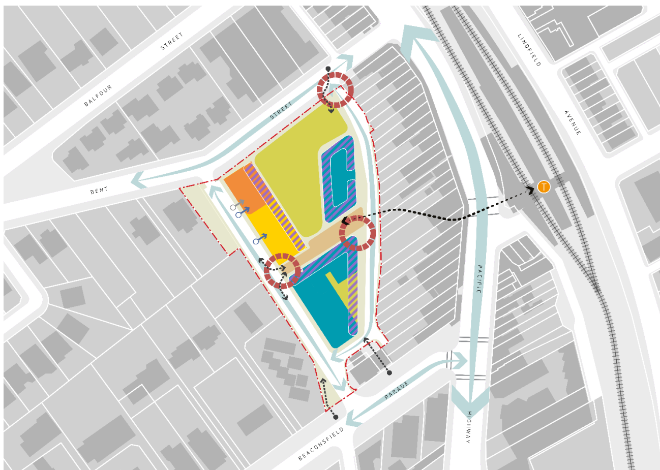
Figure 5.1 Revised masterplan indicative site layout
