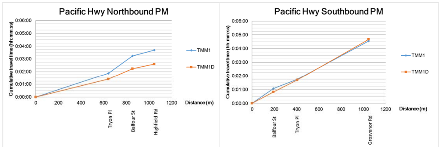
FIGURE 5 ADDITIONAL PM TRAVEL TIME COMPARISON
