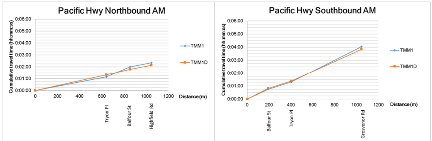
FIGURE 4 ADDITIONAL AM TRAVEL TIME COMPARISON
