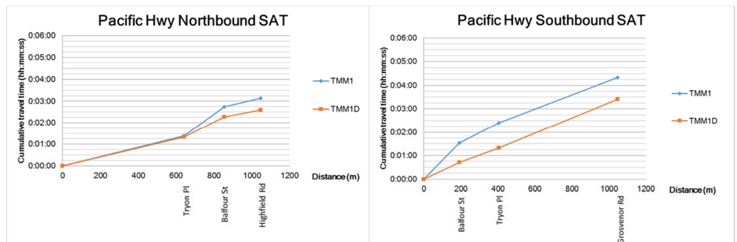
FIGURE 6 ADDITIONAL SAT TRAVEL TIME COMPARISON
