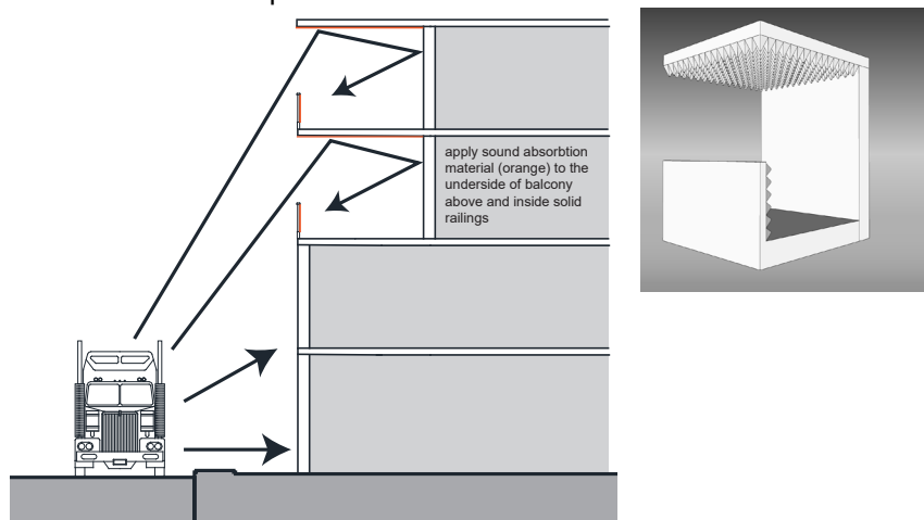
Figure 8C.15-2: Limiting reflected noise on high rise balconies and within adjacent rooms. Ku-ring-gai Development Control Plan
